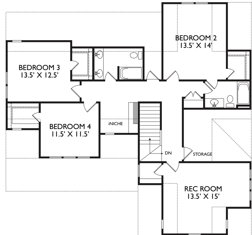
SECOND FLOOR
